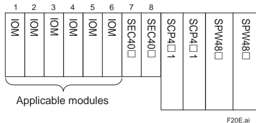
Figure Mounting examples of a safety control unit (with ESB bus coupler)
